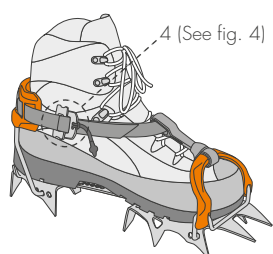
6.1 - Full lacing
